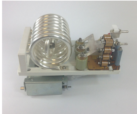
853-015130-102 | LAM Research RF Mini-Match
